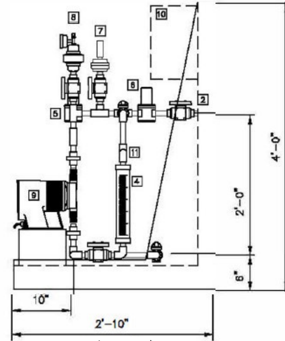
RIGHT VIEW
