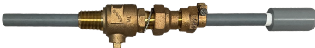
3/4" Corp Stop with a 3/8" PVC Nozzle w/1/2" FPT Connection.
